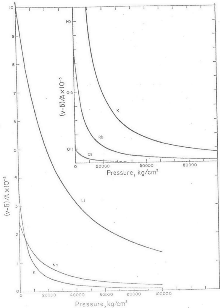
FIG. 3. Pressure vs. defect volume, (v-B) , for the alkali metals.
