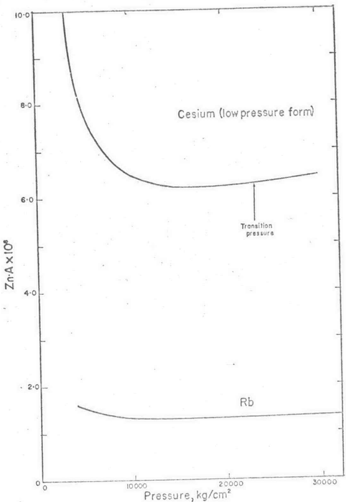
FIG. 2. Pressure vs. number-average degree of association, Zn , times A for cesium. The ZnA scale is compressed here compared to Fig. 1 and the pressure scale is expanded. The curve for rubidium is repeated for comparison.
